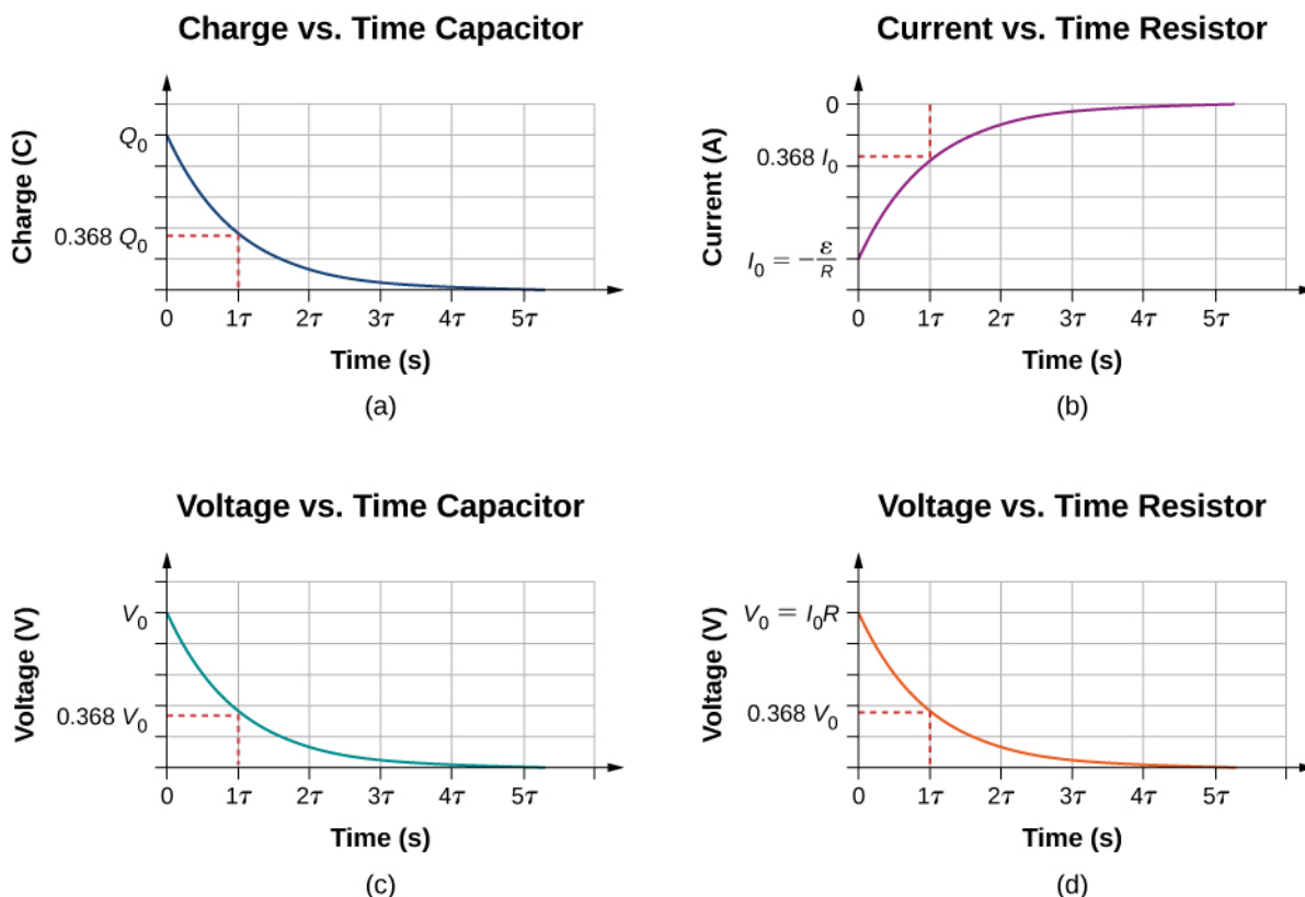
Figure 10.40 (a) Charge on the capacitor versus time as the capacitor discharges. (b) Current through the resistor versus time. (c) Voltage difference across the capacitor. (d) Voltage difference across the resistor.
