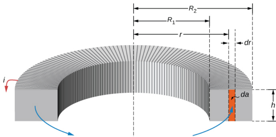
Figure 14.10 Calculating the self-inductance of a rectangular toroid.
