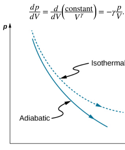
Figure 3.15 Quasi-static adiabatic and isothermal expansions of an ideal gas.
